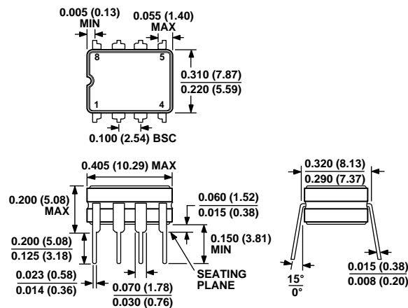
Figure 47. 8-Lead Ceramic DIP – Glass Hermetic Seal [CERDIP] (Q-8)
