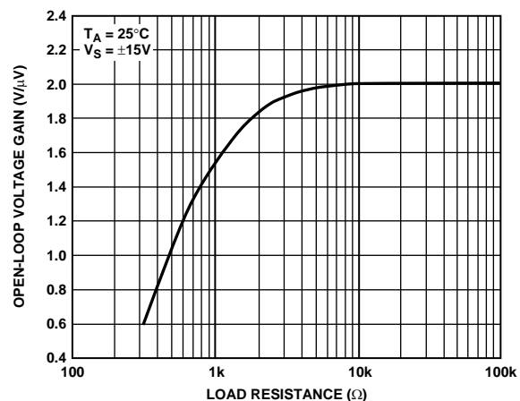
Figure 32. Open-Loop Voltage Gain vs. Load Resistance
